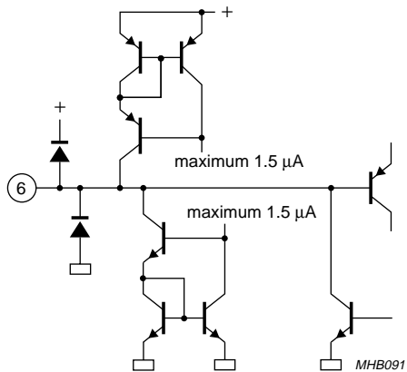
Fig.23 Pin 6 (AFD).
