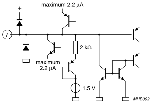
Fig.24 Pin 7 (FAGC).
