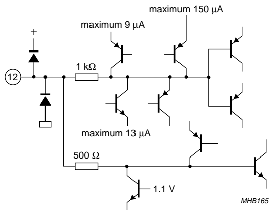
Fig.29 Pin 12 (TR).
