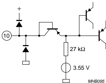
Fig.27 Pin 10 (S1).
