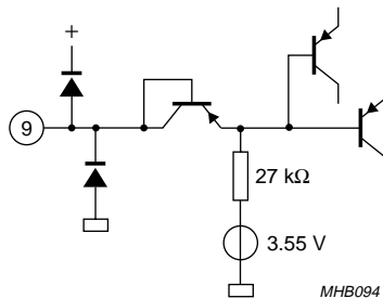
Fig.26 Pin 9 (S0).
