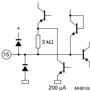
Fig.32 Pin 15 (REF).
