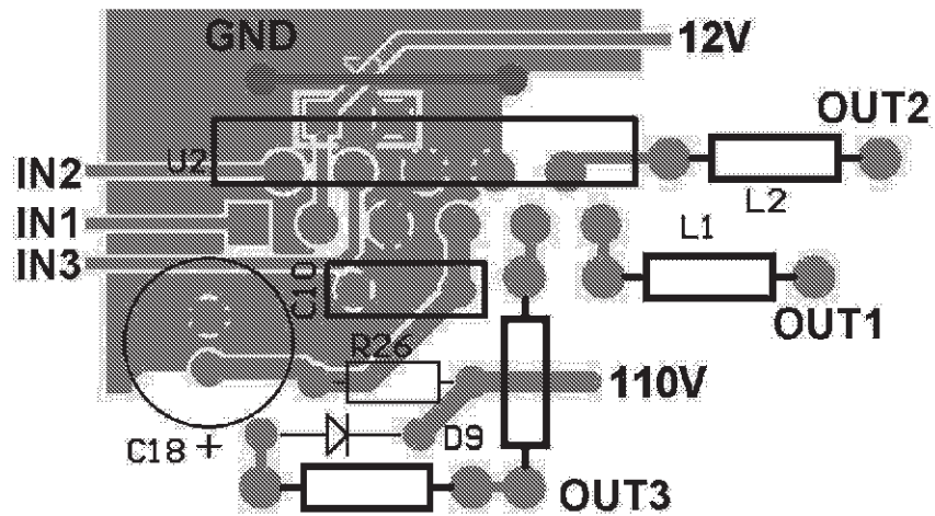
Figure 13. Amplifier and Preamplifier Outputs. Trace Routing (detail)
