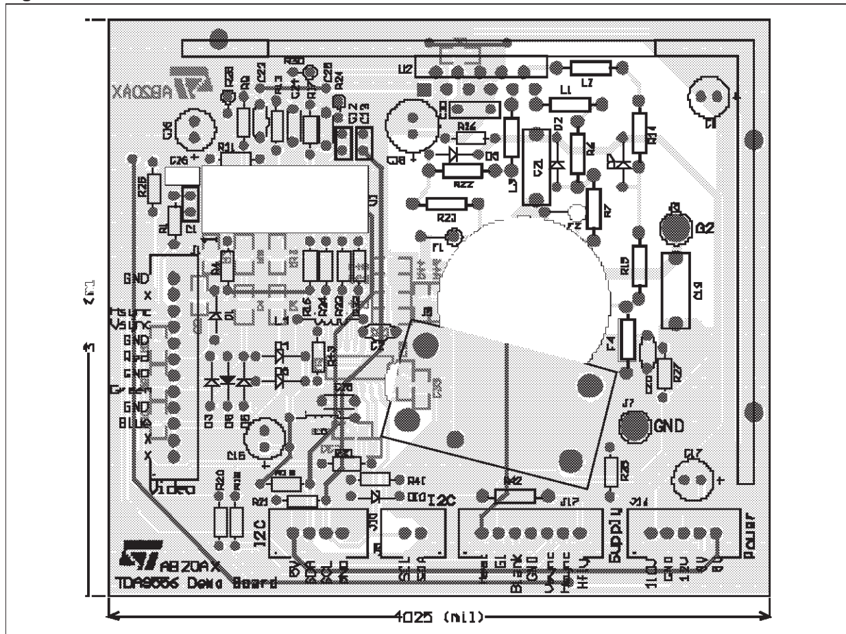
Figure 12. TDA9210 - TDA9556 - STV9935 Demonstration Board: Silk Screen and Trace
