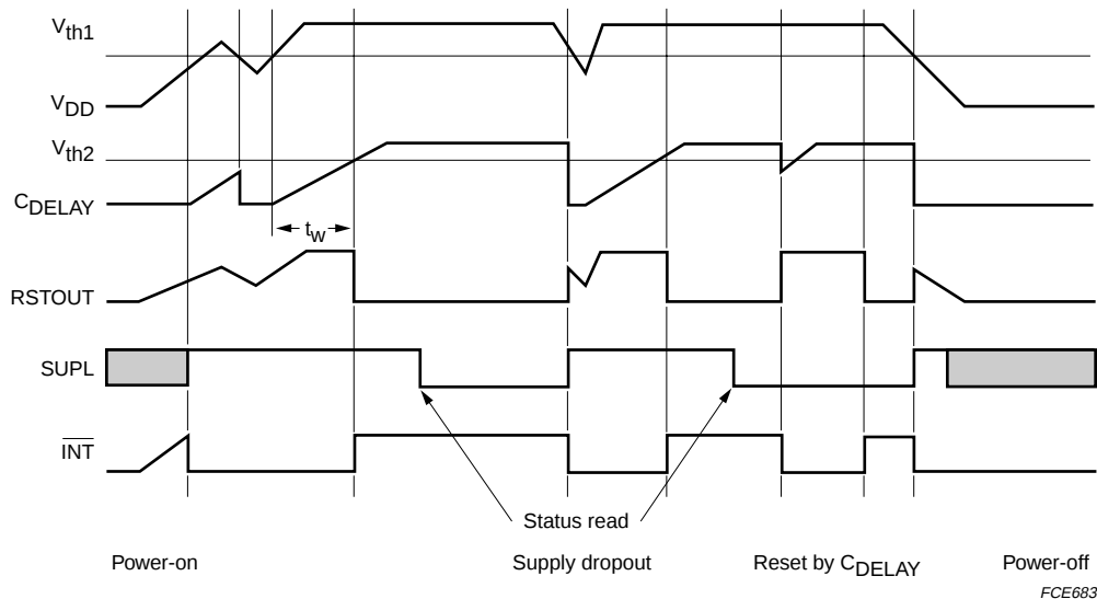
Fig.7 Voltage supervisor.
