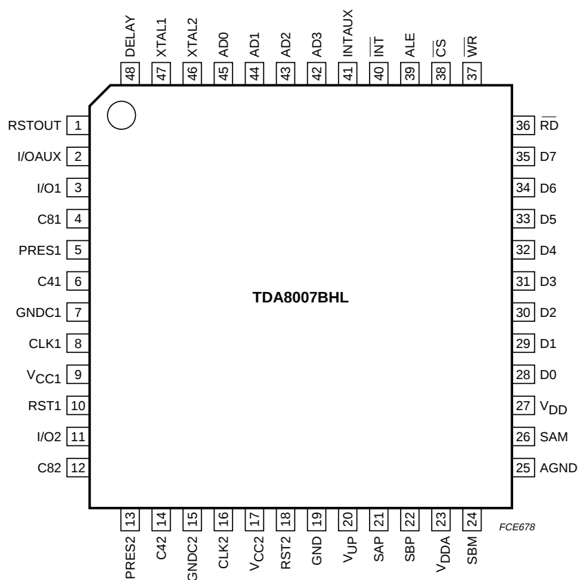
Fig.2 Pin configuration.
