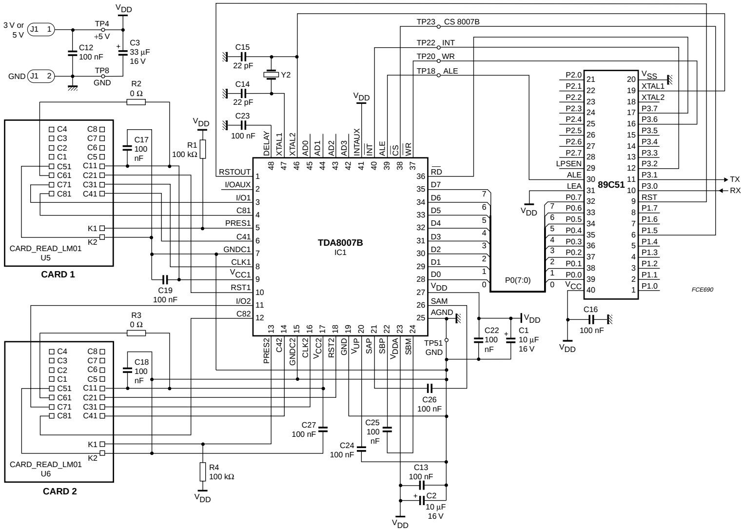
Fig.10 Application diagram.
