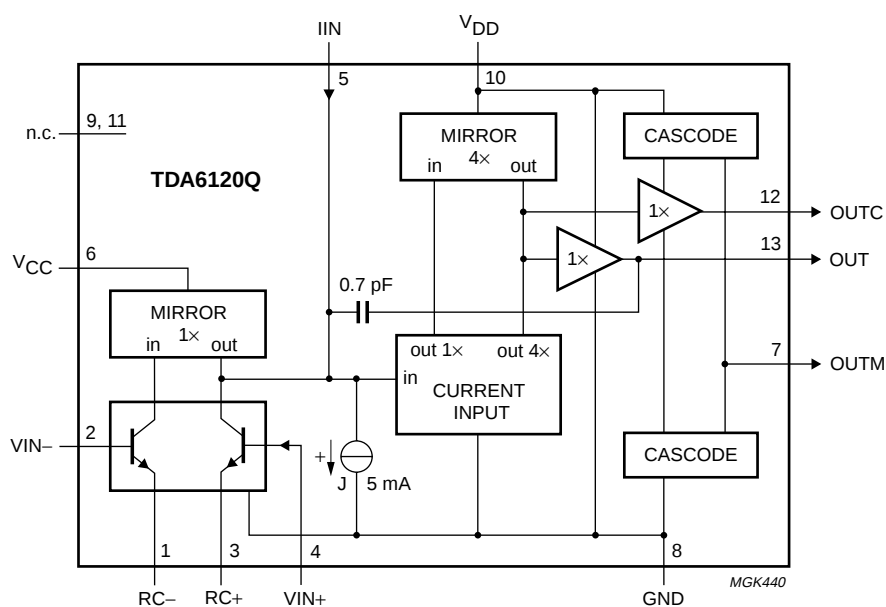
Fig.1 Block diagram.
