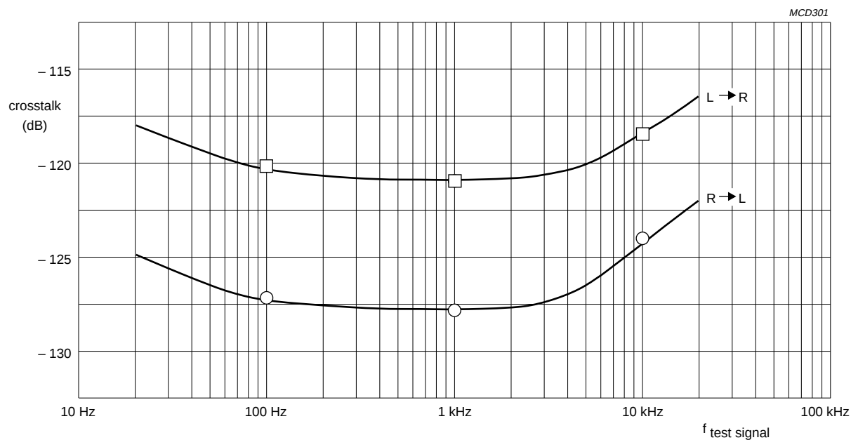
Fig.9 Inter-channel crosstalk as a function of signal frequency.
