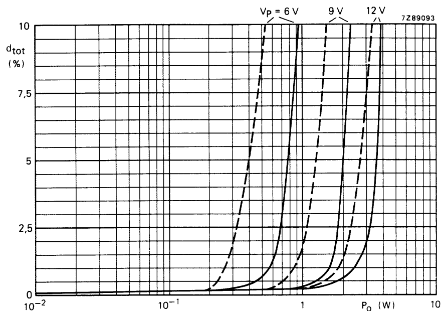
Fig.6 Total harmonic distortion as a function of output power across R_L ; — with bootstrap; - - - without bootstrap; f = 1\text{ kHz} ; typical values. The available output power is 5% higher when measured at pin 2 (due to series resistance of C10).
