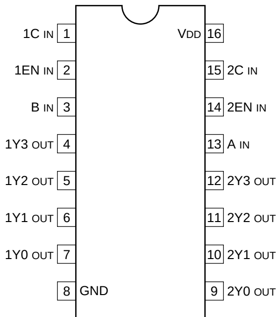
DUAL 2-TO-4-LINE DECODER
