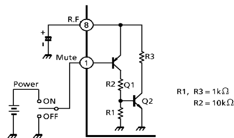
Fig.4 Mute circuit
