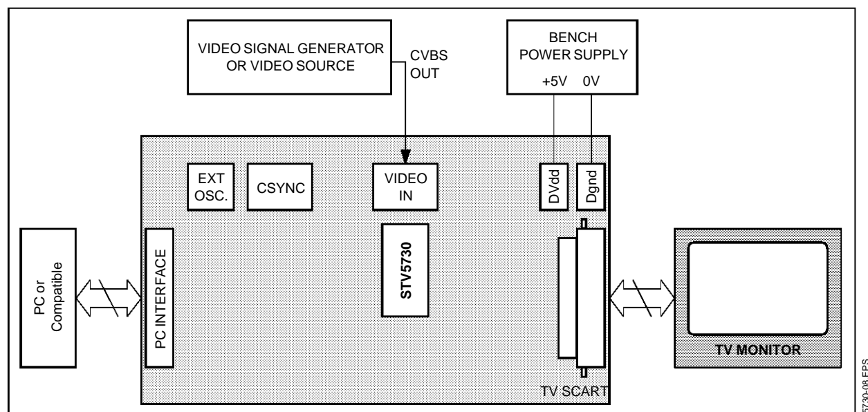
Figure 1 : STV5730 Evaluation Connection Diagram
