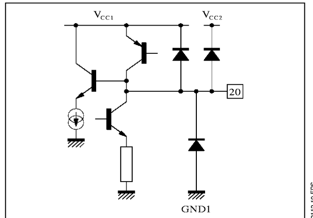
Figure 17 : Pin 20 - Y/CVBS
