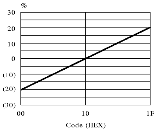
Figure 5 : Volume Control Curve
