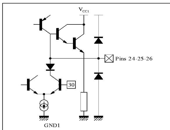
Figure 21 : Pin 30 - ICAT
