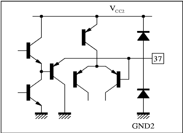
Figure 28 : Pin 37 - LFB/SC
