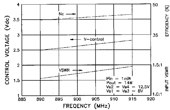
CONTROL VOLTAGE, EFFICIENCY &amp; INPUT VSWR vs FREQUENCY
