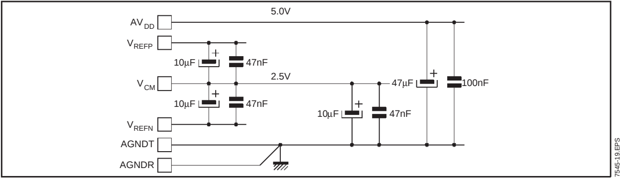
Figure 17 : Voltage Decoupling
