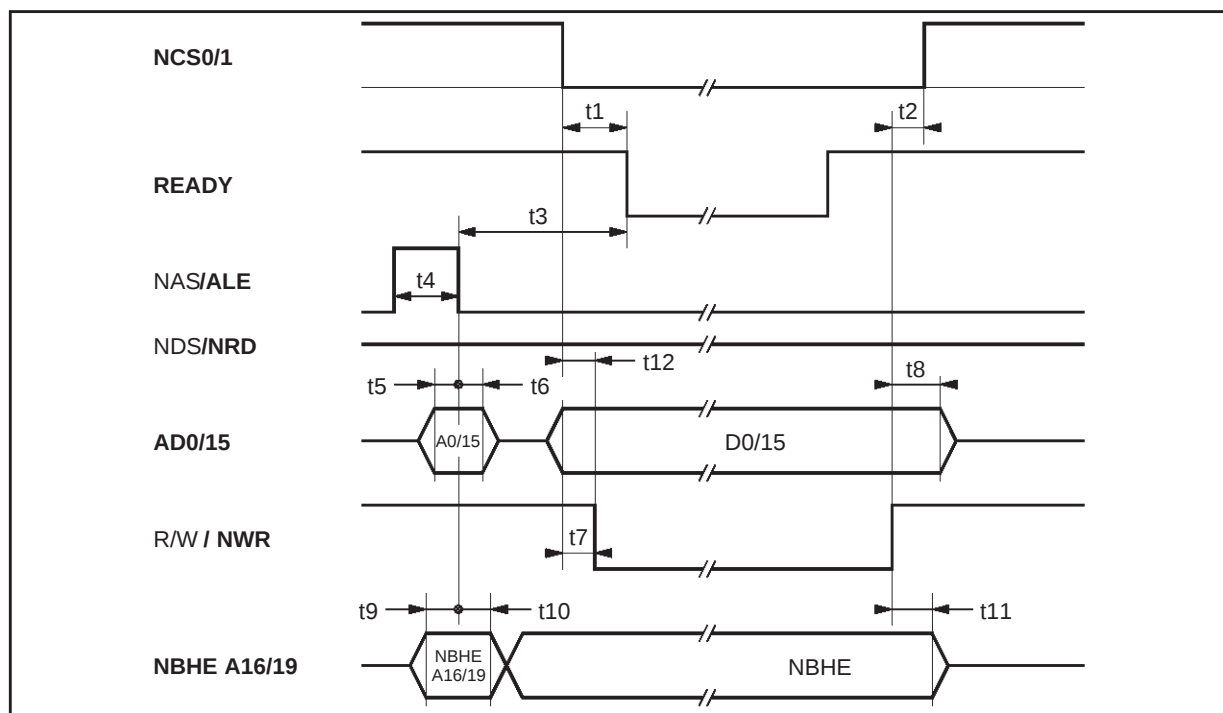
Figure 51 : 80C186 Write Cycle
