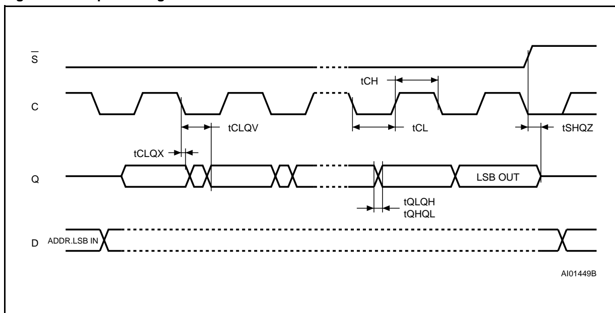
Figure 15. Output Timing
