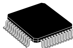
TQFP48 (7 x 7 x 1.40mm) (Full Plastic Quad Flat Pack) ORDER CODE : ST7554TQF7
