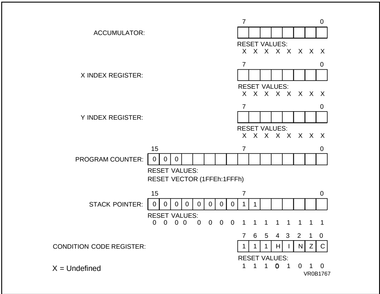
Figure 4. Organisation of Internal CPU Registers
