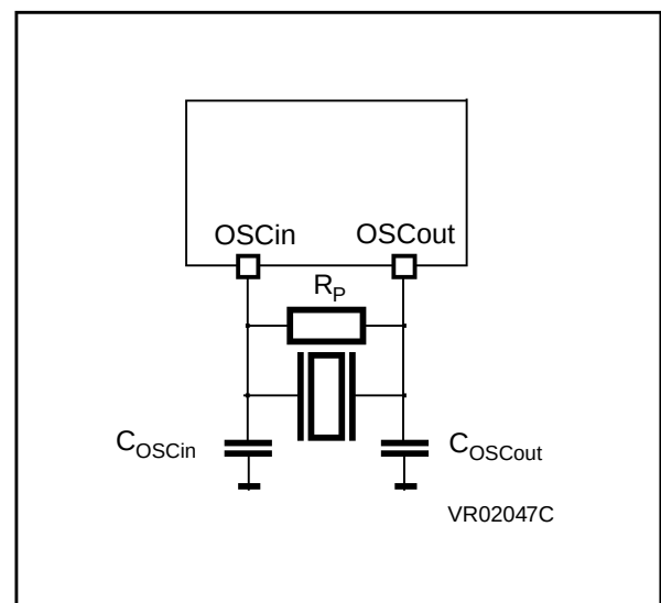
Figure 8. Crystal/Ceramic Resonator
