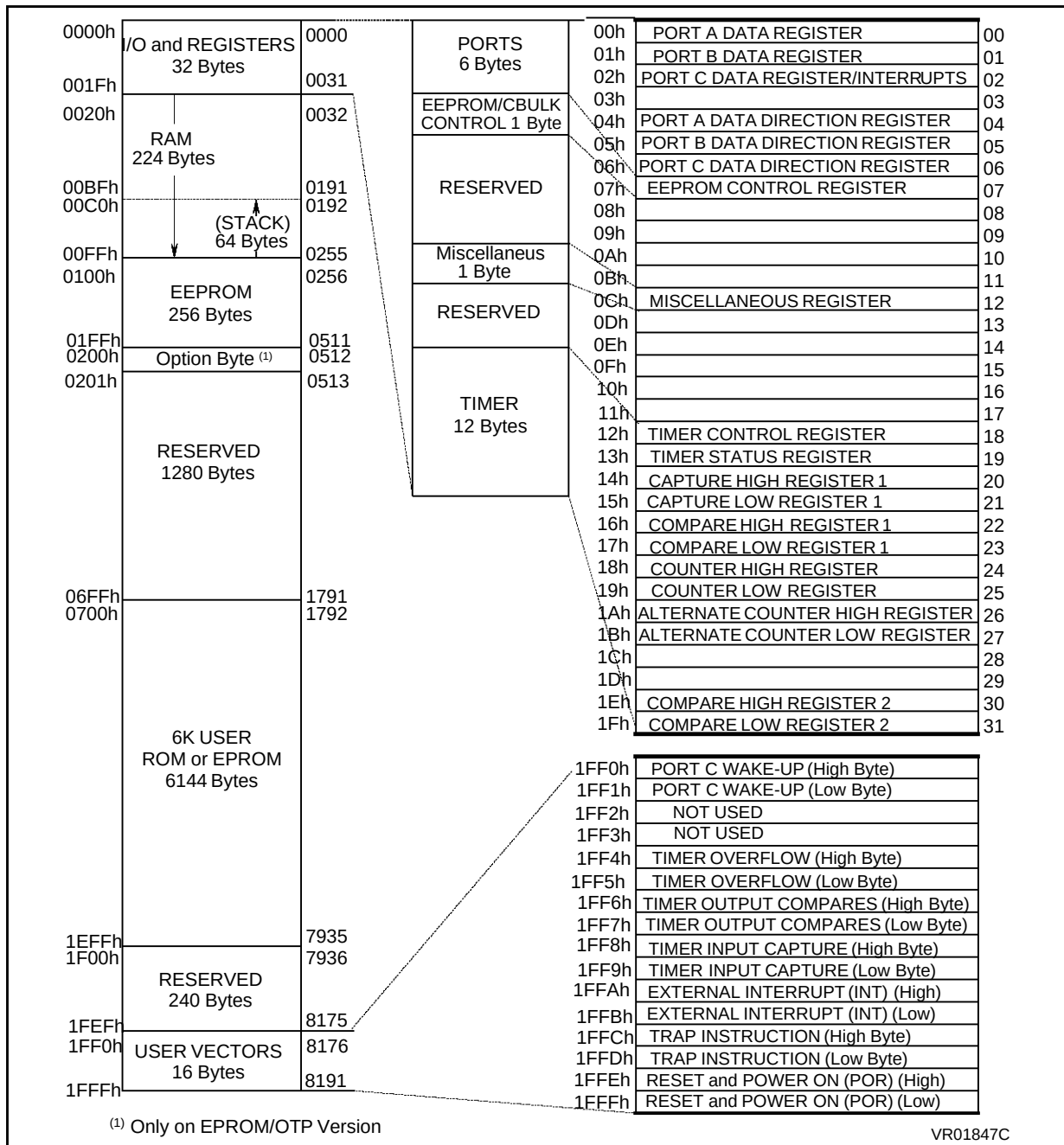
Figure 3. Memory Map
