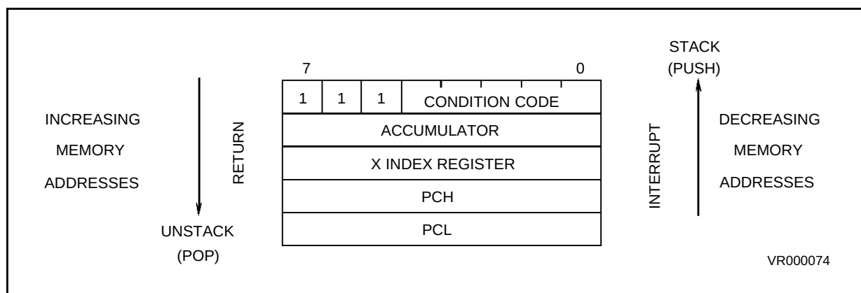
Figure 5. Stacking Order
