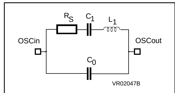
Figure 8. Crystal/Ceramic Resonator
