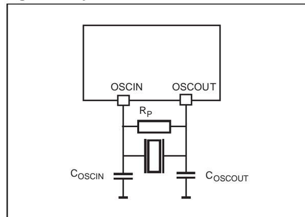
Figure 8. Crystal/Ceramic Resonator
