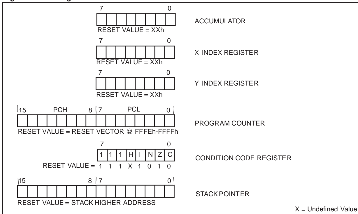
Figure 6. CPU Registers
