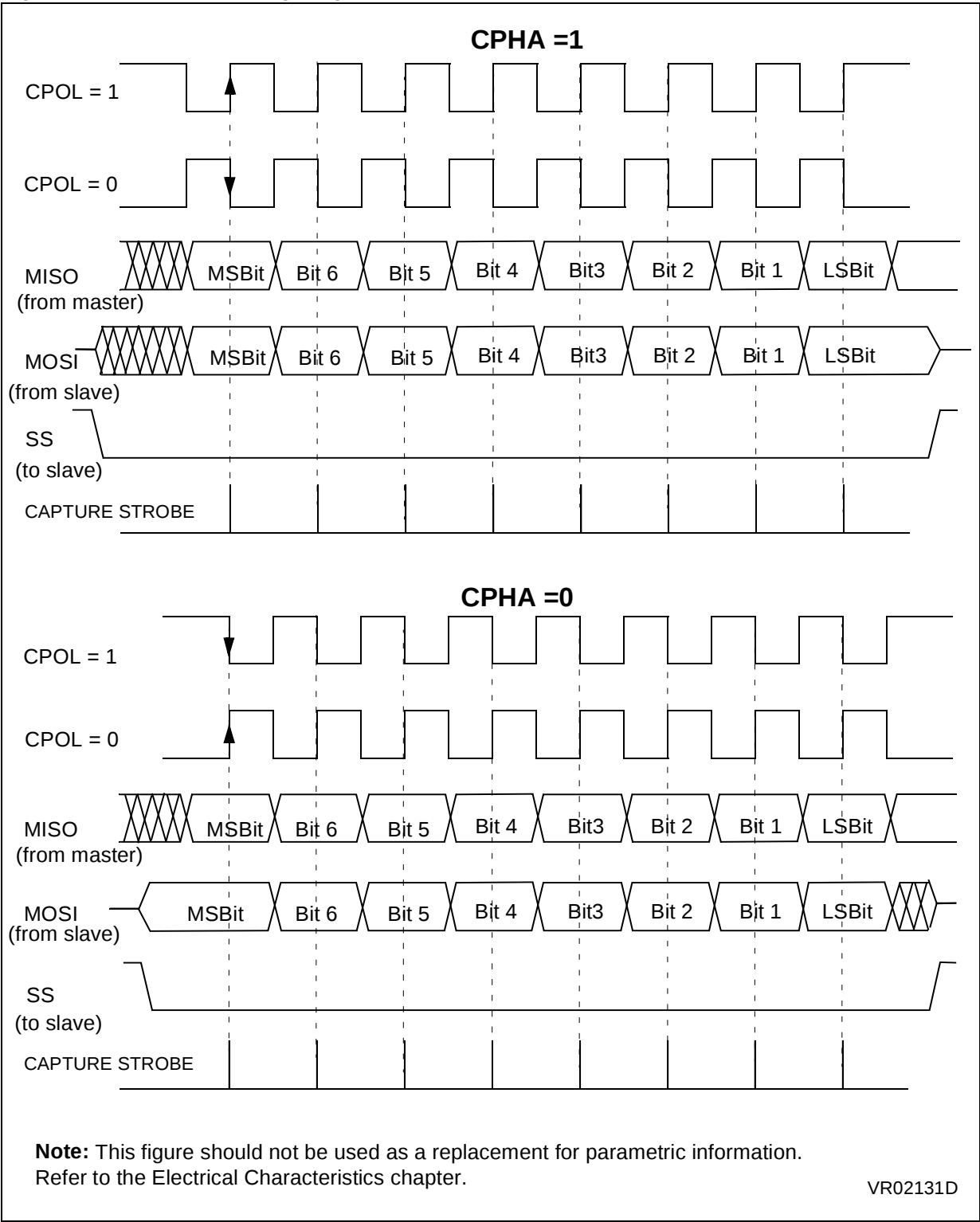
Figure 42. Data Clock Timing Diagram
