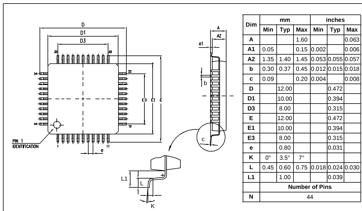
Figure 58. 44-Pin Thin Quad Flat Package
