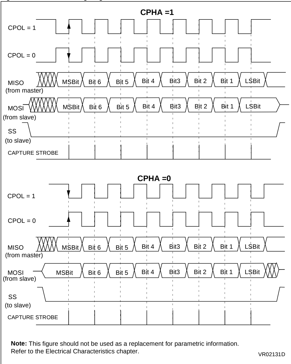
Figure 39. Data Clock Timing Diagram
