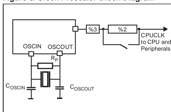
Figure 8. Clock Prescaler Block Diagram
