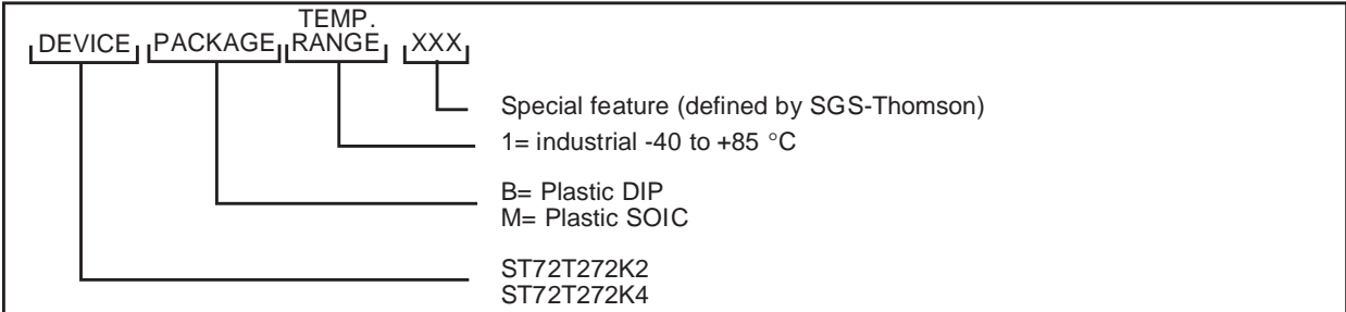
Figure 43. OTP User Programmable Device Types
