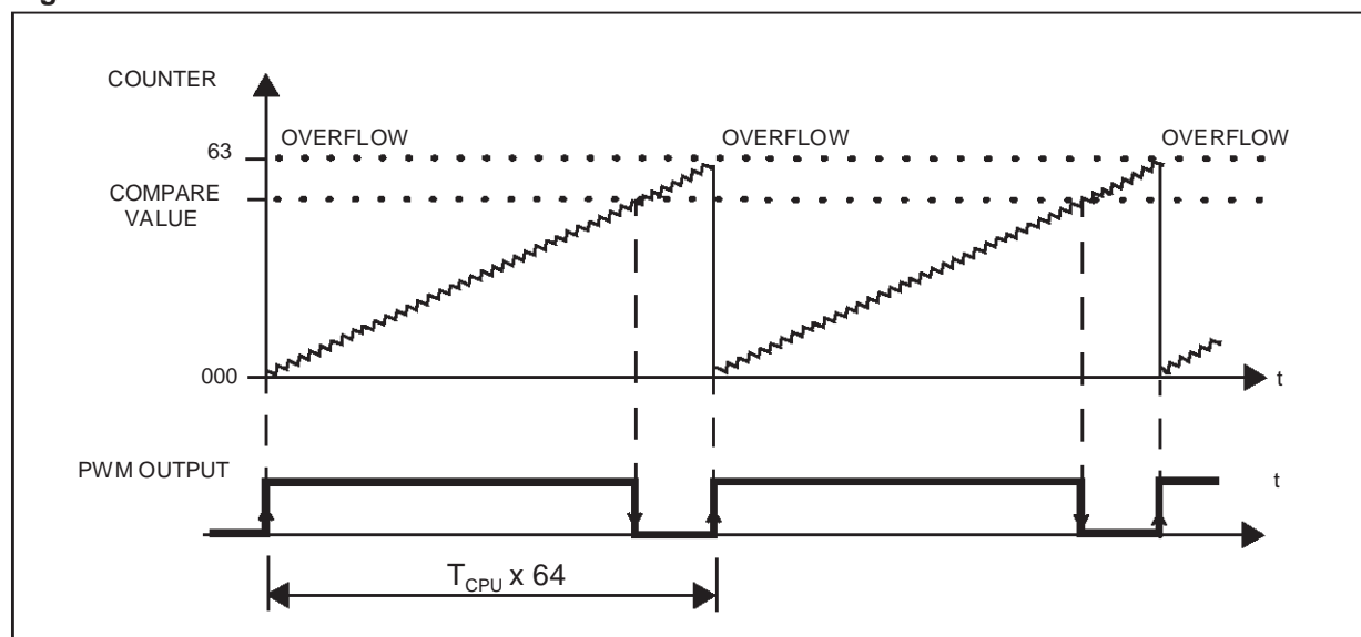
Figure 30. PWM Generation
