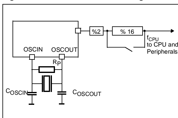
Figure 9. Clock Prescaler Block Diagram
