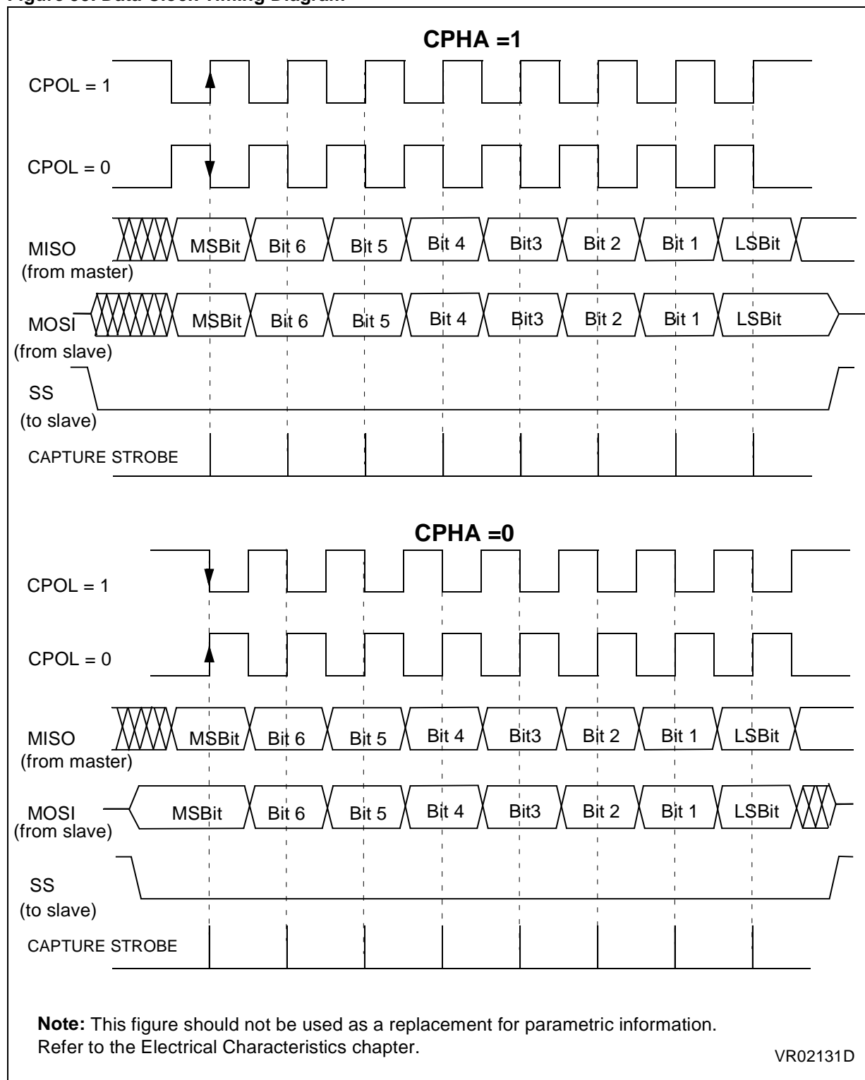
Figure 35. Data Clock Timing Diagram
