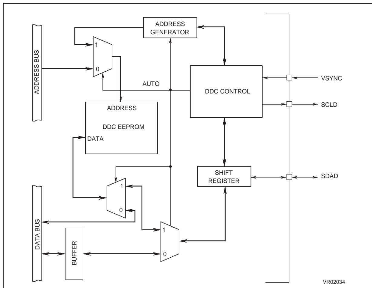
Figure 29. DDC SPI Block Diagram
