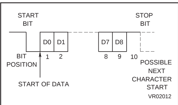
Figure 25. Character Format
