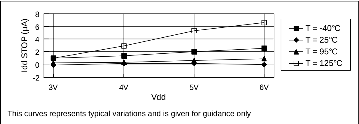
Figure 44. Idd STOP versus Vcc for ROM devices
