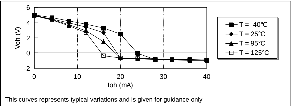
Figure 90. Voh versus Ioh on all I/O port at Vdd=5V
