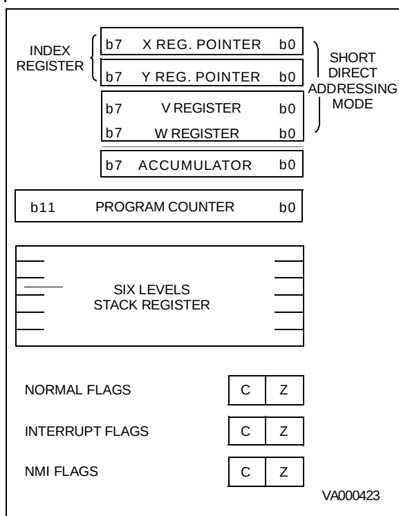
Figure 50. ST6 CPU Programming Mode
