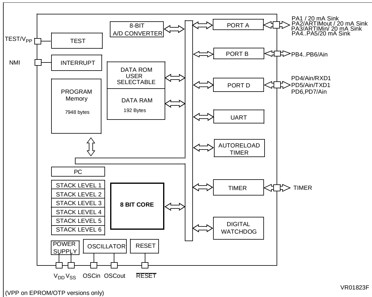
Figure 44. Block Diagram
