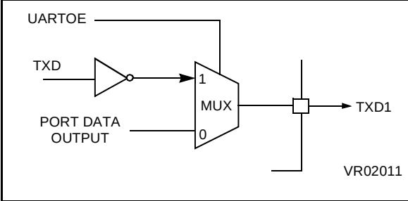
Figure 75. UART Data Output
