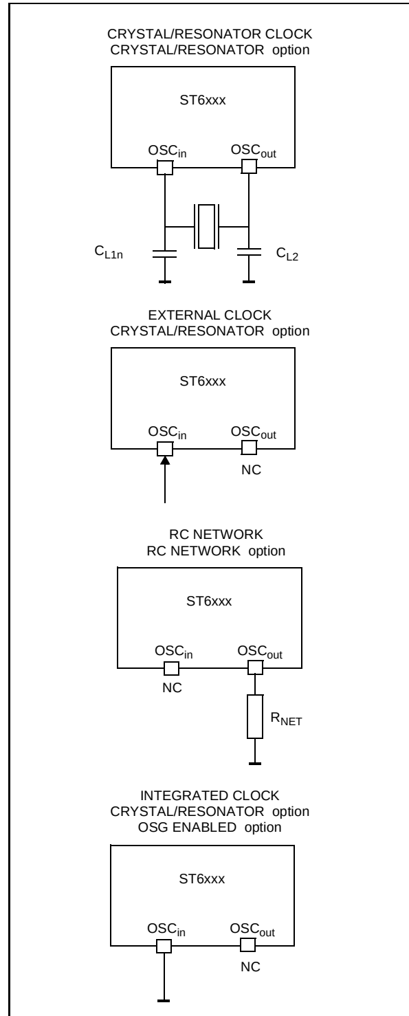
Figure 51. Oscillator Configurations
