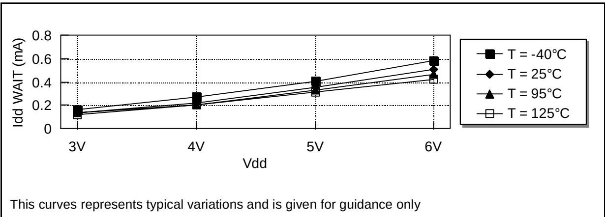
Figure 84. Idd RUN versus Vcc at 8 Mhz for ROM and OTP devices
