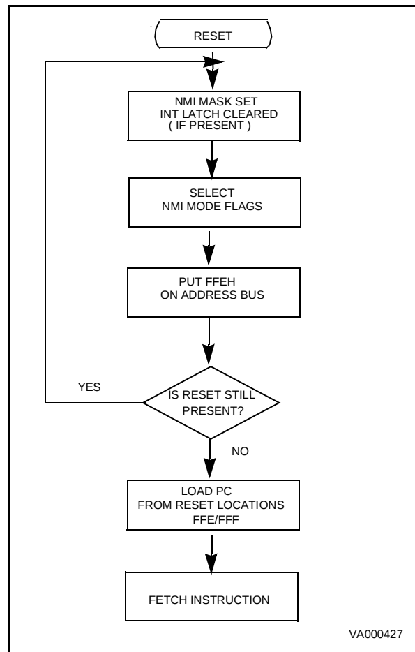
Figure 56. Reset and Interrupt Processing
