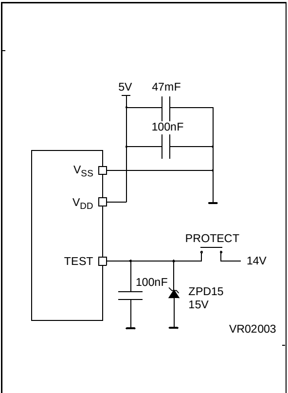
Figure 1. Programming Circuit
