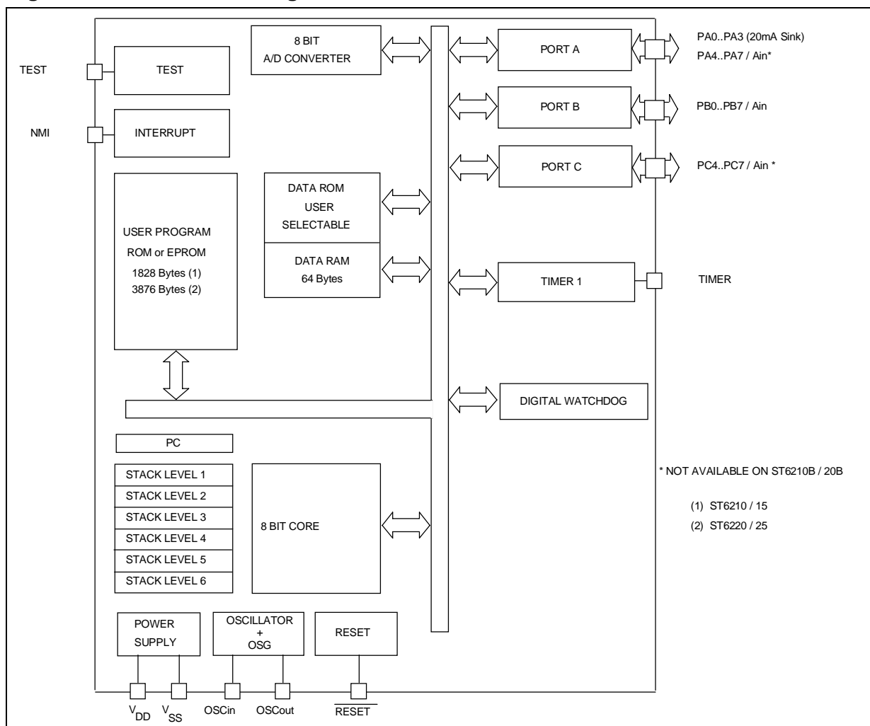
Figure 18. ST6220 Block diagram
