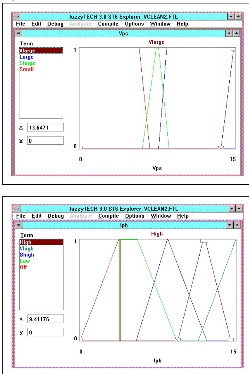
Figure 5. Membership Functions for Pressure(Vps) & Peak
