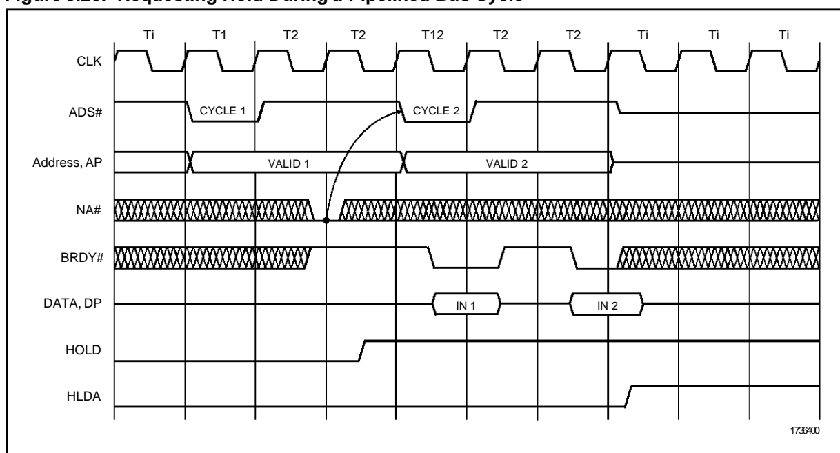
Figure 3.20. Requesting Hold During a Pipelined Bus Cycle
