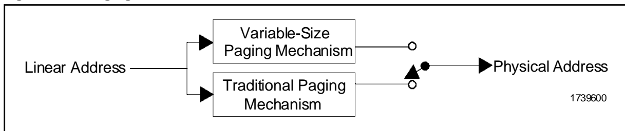
Figure 2.29. Paging Mechanisms
