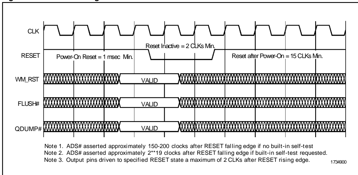
Figure 3.2. RESET Timing
