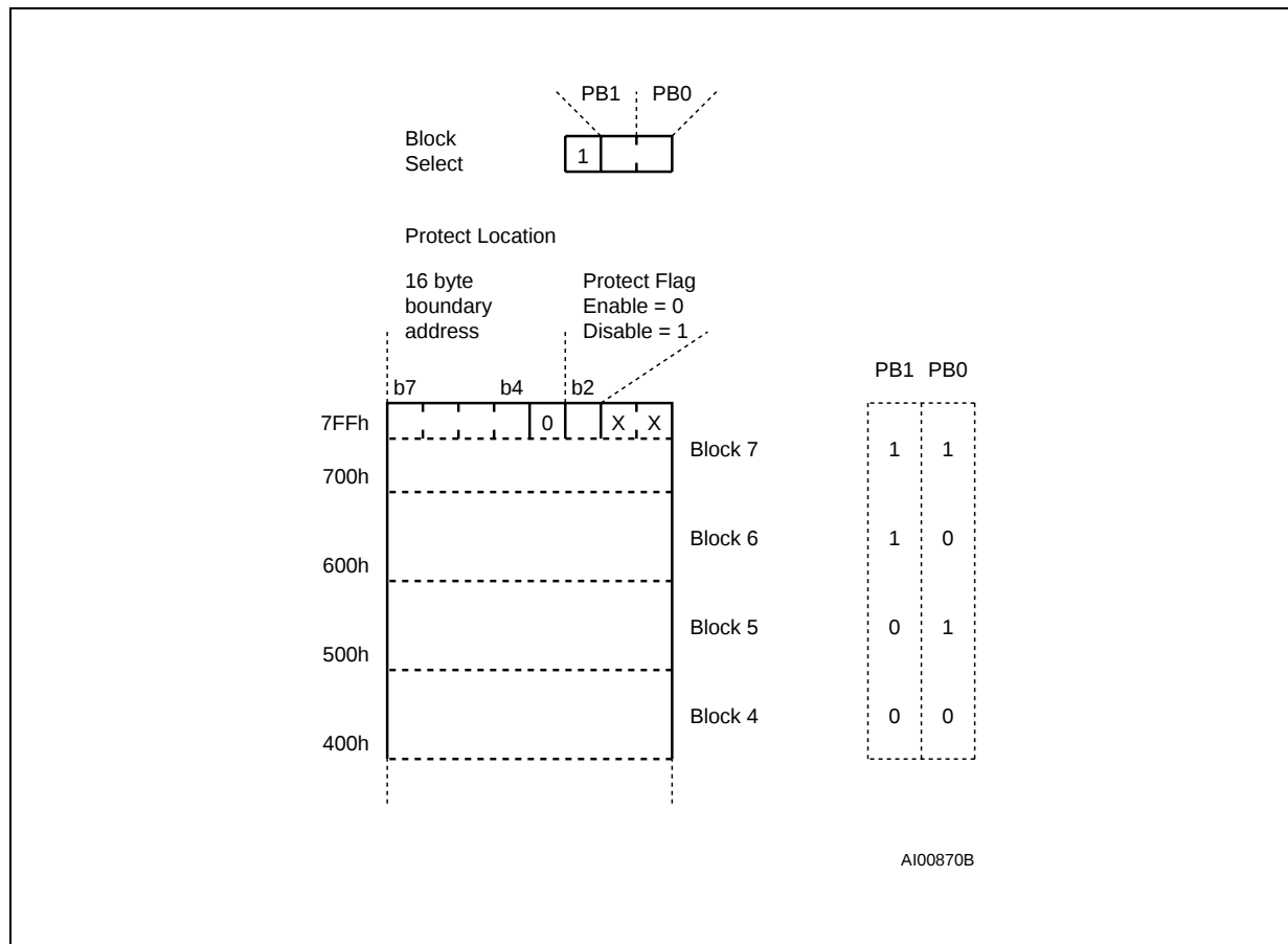
Figure 7. Memory Protection
