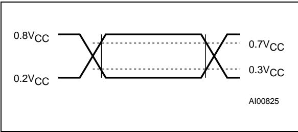
Figure 8. AC Testing Input Output Waveforms
