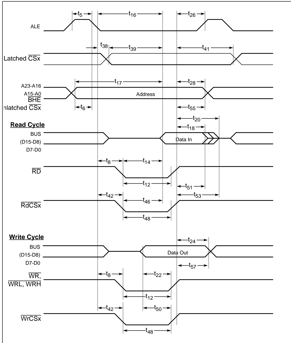
Figure 18 External memory cycle: demultiplex bus, with read/write delay, normal ALE
