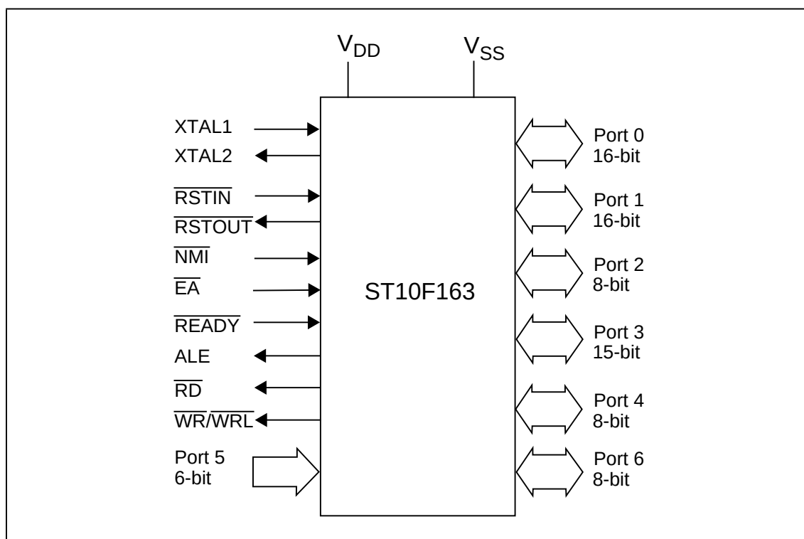
Figure 1 Logic symbol
