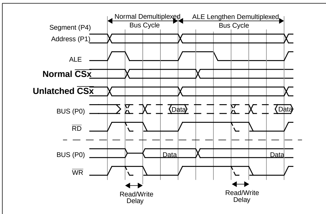
Figure 4 Chip select delay
