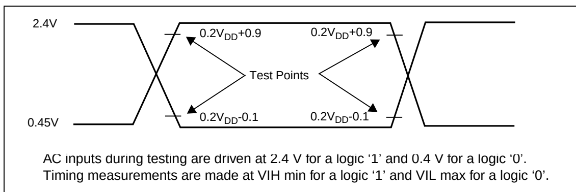
Figure 9 Input/output waveforms
