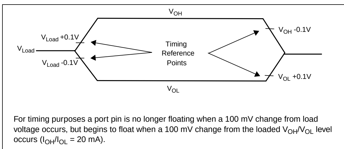
Figure 10 Float waveforms
