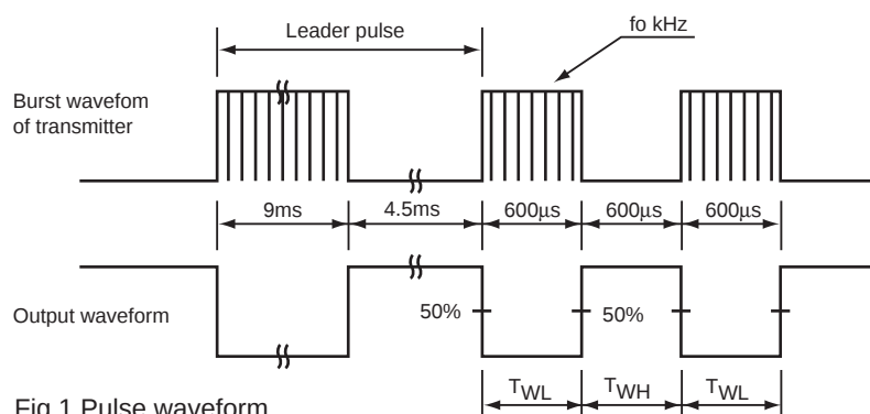
Fig.1 Pulse waveform
