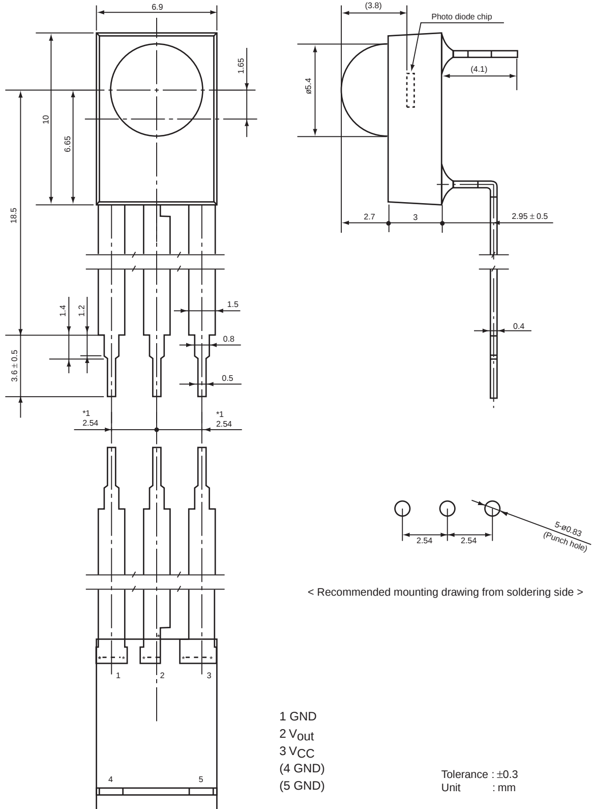
SPS-445 Series Package Dimensions and Pinconnection
