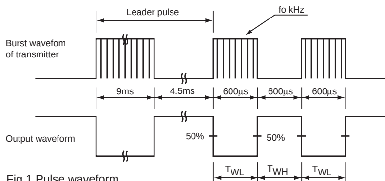
Fig.1 Pulse waveform
