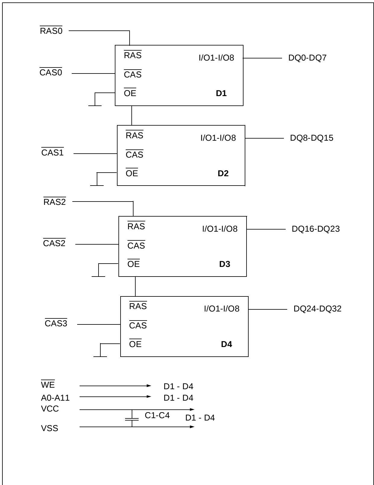
Block Diagram
