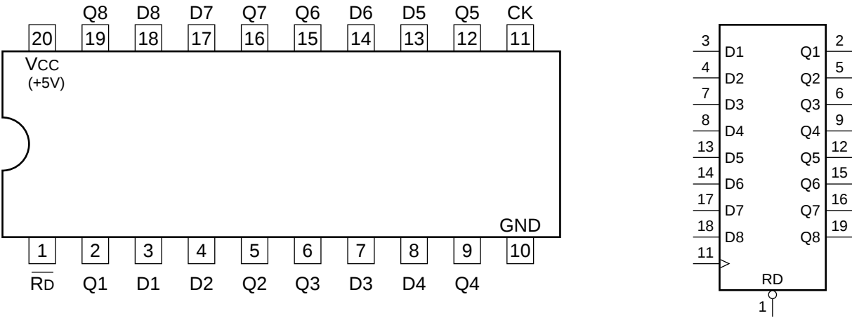
EACH FLIP-FLOP
