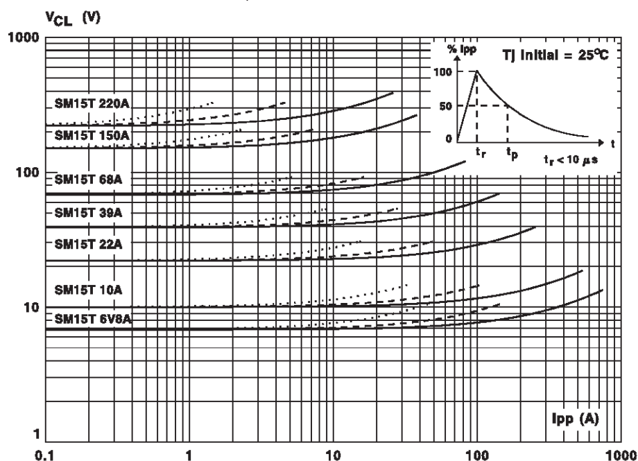
Fig. 3 : Clamping voltage versus peak pulse current. Exponential waveform t_p = 20 \mu\text{s} ——— t_p = 1 \text{ ms} - - - - - t_p = 10 \text{ ms} .....
