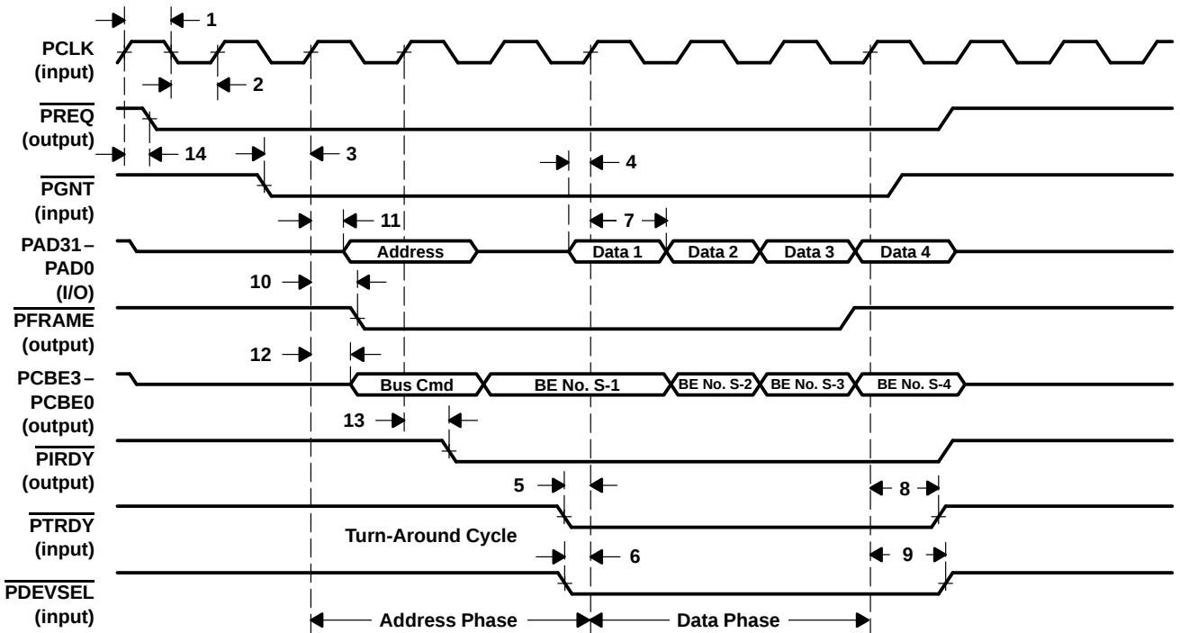
Figure 4. TNETA1561 Read Operation (PCI SAR as Master)
