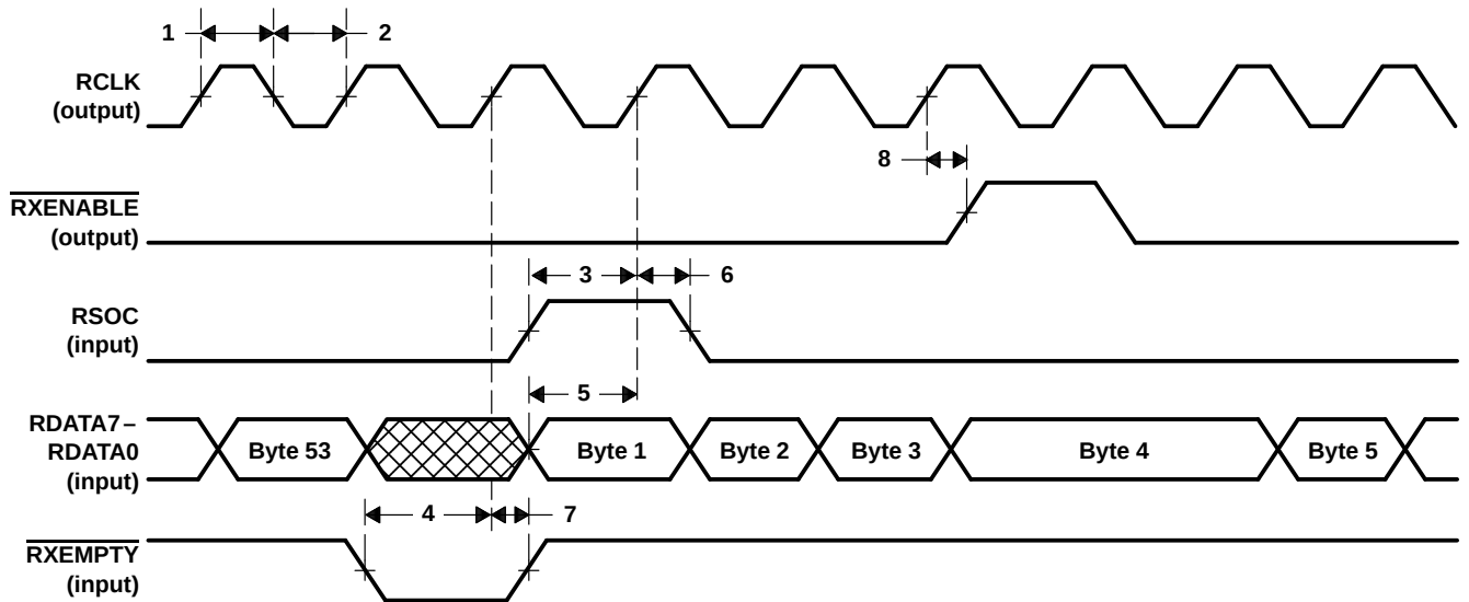
Figure 1. Receive-Cell Interface
