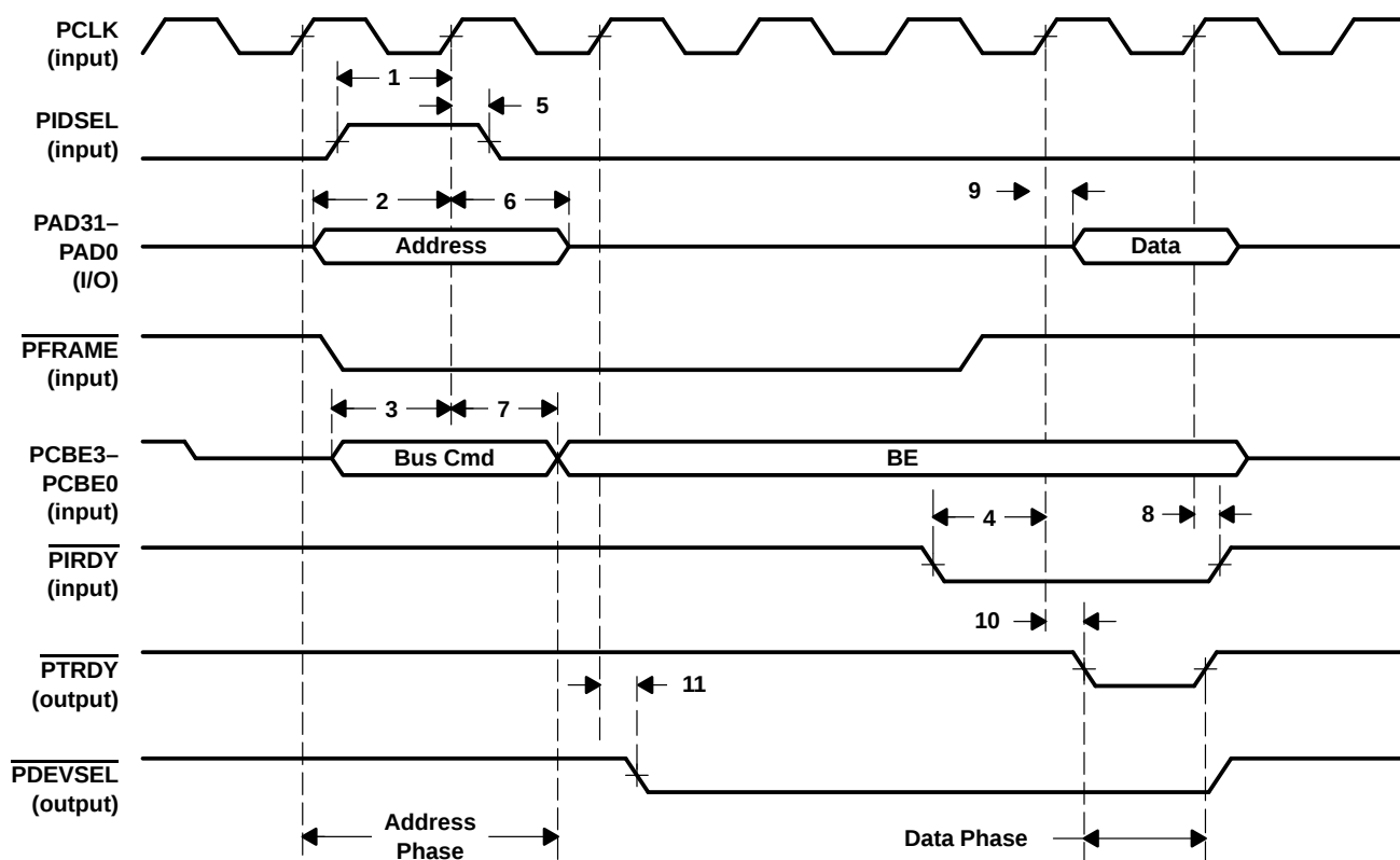
Figure 5. TNETA1561 Read Operation (PCI SAR as Slave)
