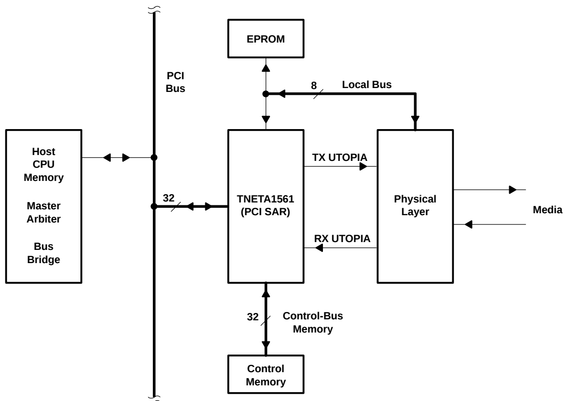
Figure 11. TNETA1561 Architecture
