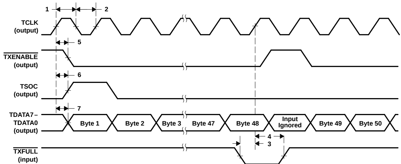
Figure 2. Transmit-Cell Interface
