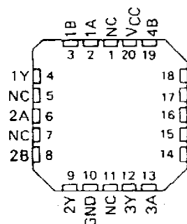
SN54LS132, SN54S132 . . . FK PACKAGE (TOP VIEW)
