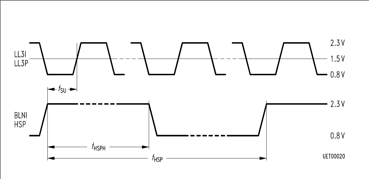
Timing Diagram 3
