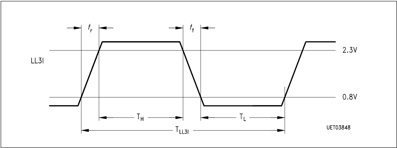
Timing Diagram 1
