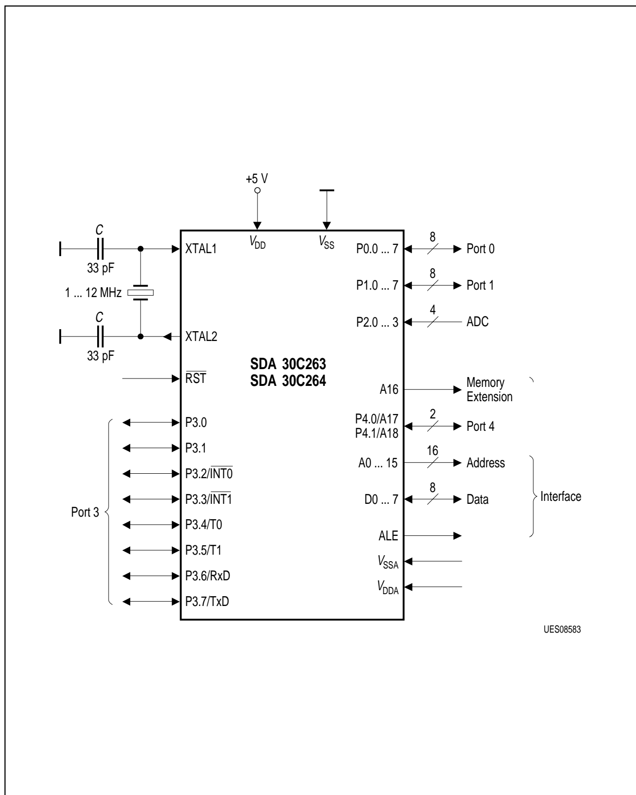
Figure 31 Application Circuit
