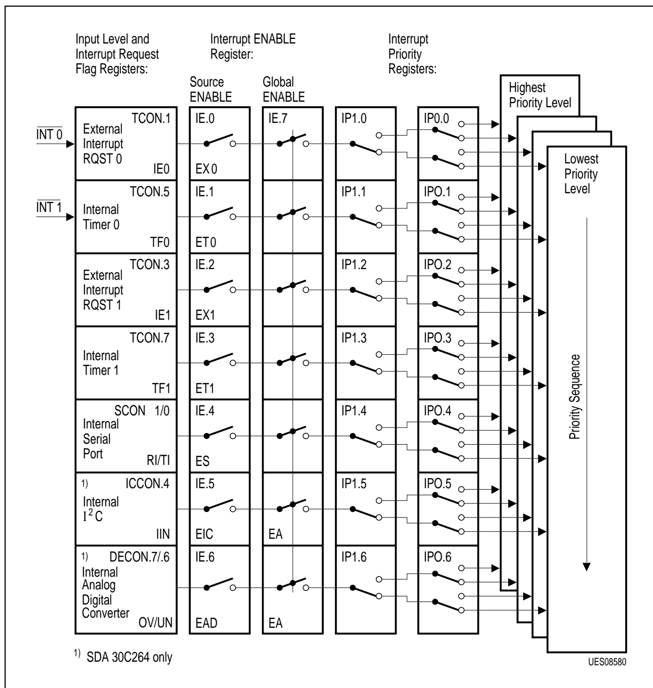
Figure 13 Interrupt System
