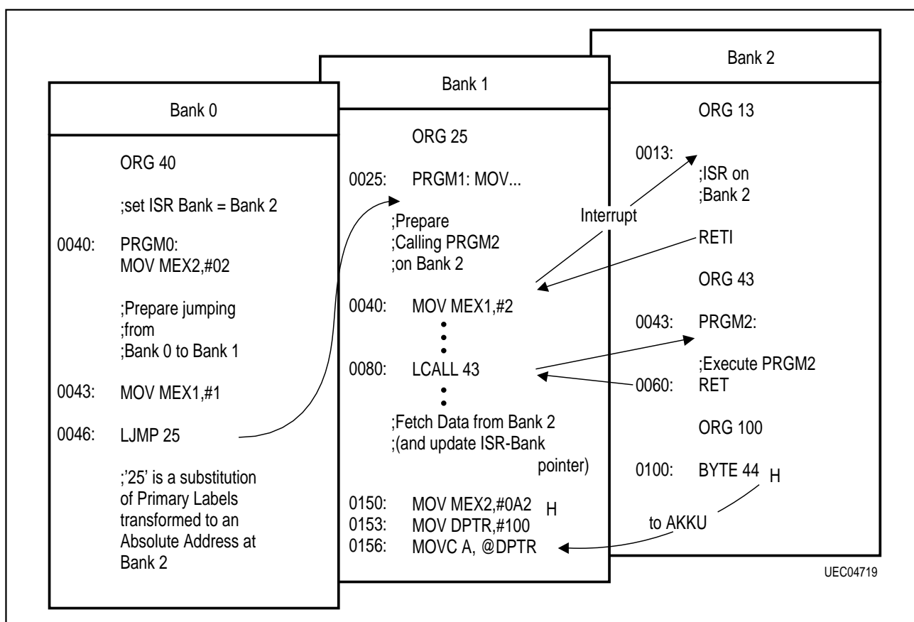
Figure 9 Program Example
