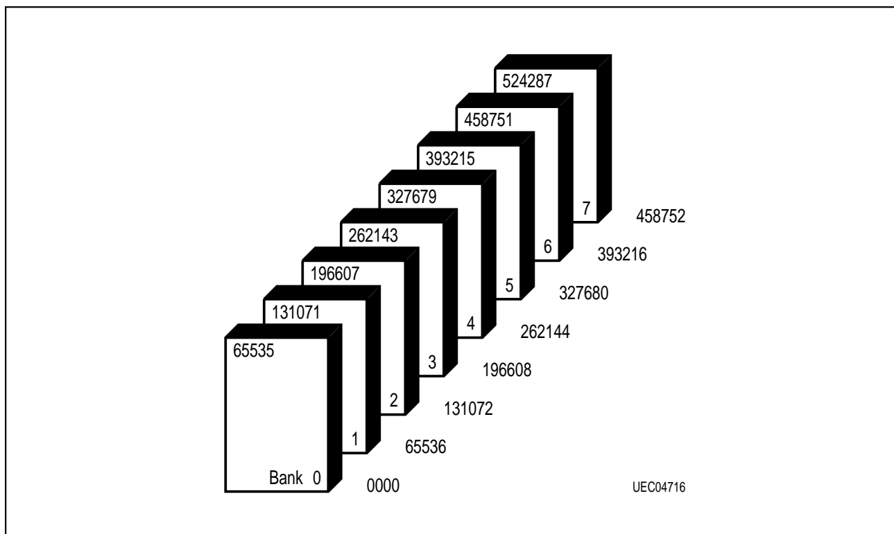
Figure 5 Bank Organization
