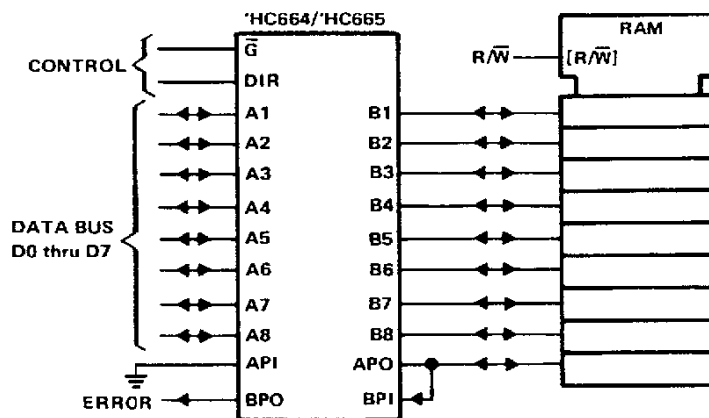
FIGURE 2. 8-BIT-WIDE MEMORY ARRAY WITH PARITY
