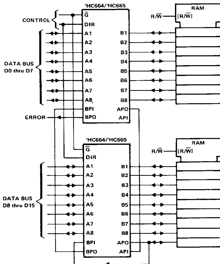
FIGURE 3. 16-BIT-WIDE MEMORY ARRAY WITH PARITY
