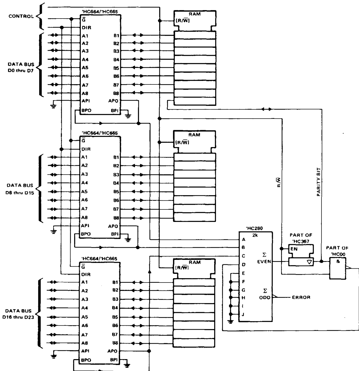
FIGURE 4. 24-BIT-WIDE MEMORY ARRAY WITH PARITY
