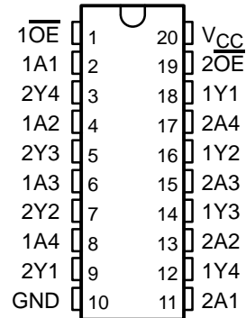
SN54BCT2244 . . . J OR W PACKAGE SN74BCT2244 . . . DW OR N PACKAGE (TOP VIEW)
