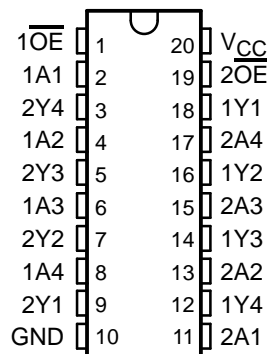
SN54ACT244 . . . J OR W PACKAGE SN74ACT244 . . . DB, DW, N, OR PW PACKAGE (TOP VIEW)
