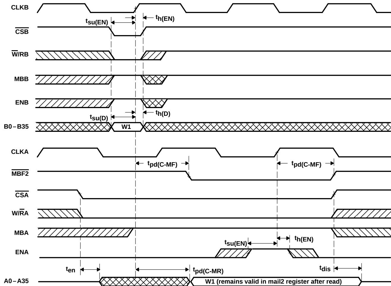
Figure 15. Timing for Mail2 Register and MBF2 Flag
