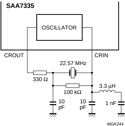
Fig.4 22.57 MHz overtone configuration.
