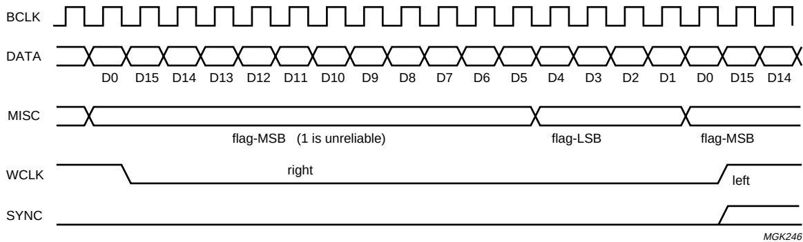
Fig.7 EIAJ ('S') data format 2 (16-bit word length).
