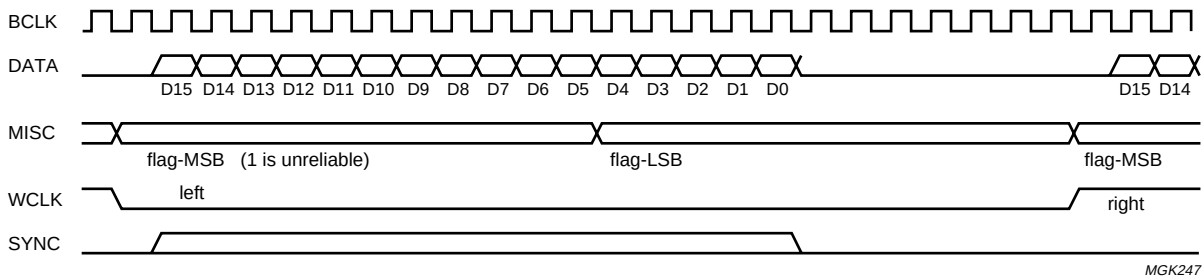
Fig.8 Philips I²S-bus data format 3 (24-bit word length).
