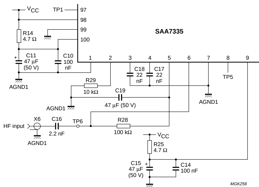
Fig.22 ADC application circuit.
