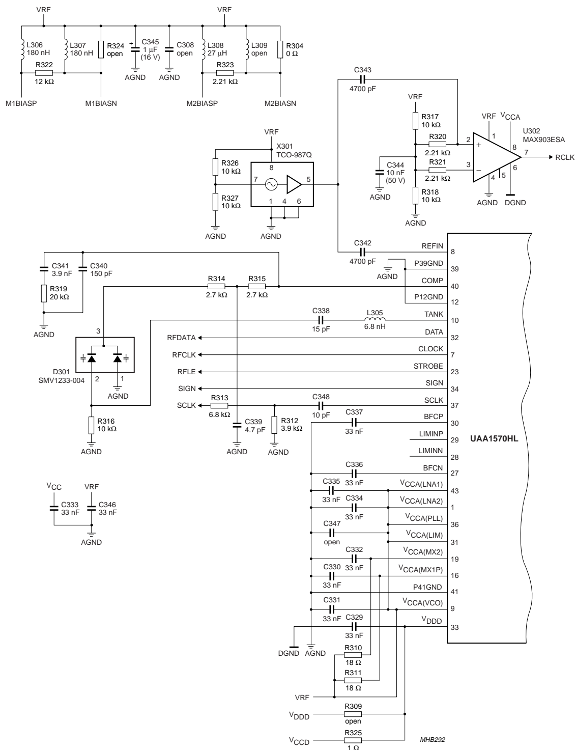
Fig.25 RF front-end circuit (continued in Fig.26).
