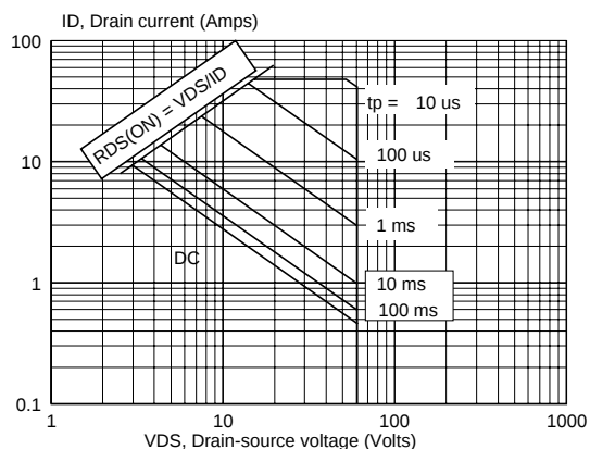
Fig.3. Safe operating area. T_{hs} = 25^\circ C I_D \text{ \& } I_{DM} = f(V_{DS}); I_{DM} \text{ single pulse; parameter } t_p
