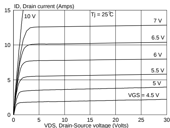
Fig.5. Typical output characteristics. I_D = f(V_{DS}); \text{ parameter } V_{GS}
