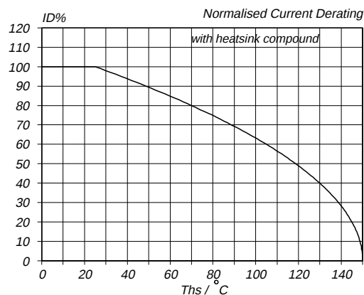
Fig.2. Normalised continuous drain current. ID\% = 100 \cdot I_D / I_{D\ 25^\circ C} = f(T_{hs}); \text{ conditions: } V_{GS} \geq 10\text{ V}
