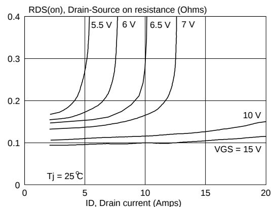
Fig.6. Typical on-state resistance. R_{DS(on)} = f(I_D); \text{ parameter } V_{GS}
