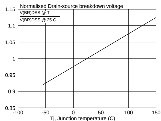
Fig.15. Normalised drain-source breakdown voltage; V_{(BR)DSS}/V_{(BR)DSS\ 25^\circ\text{C}} = f(T_j)
