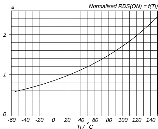
Fig.9. Normalised drain-source on-state resistance. a = R_{DS(ON)}/R_{DS(ON)25^\circ\text{C}} = f(T_J) ; I_D = 6.2 \text{ A} ; V_{GS} = 10 \text{ V}
