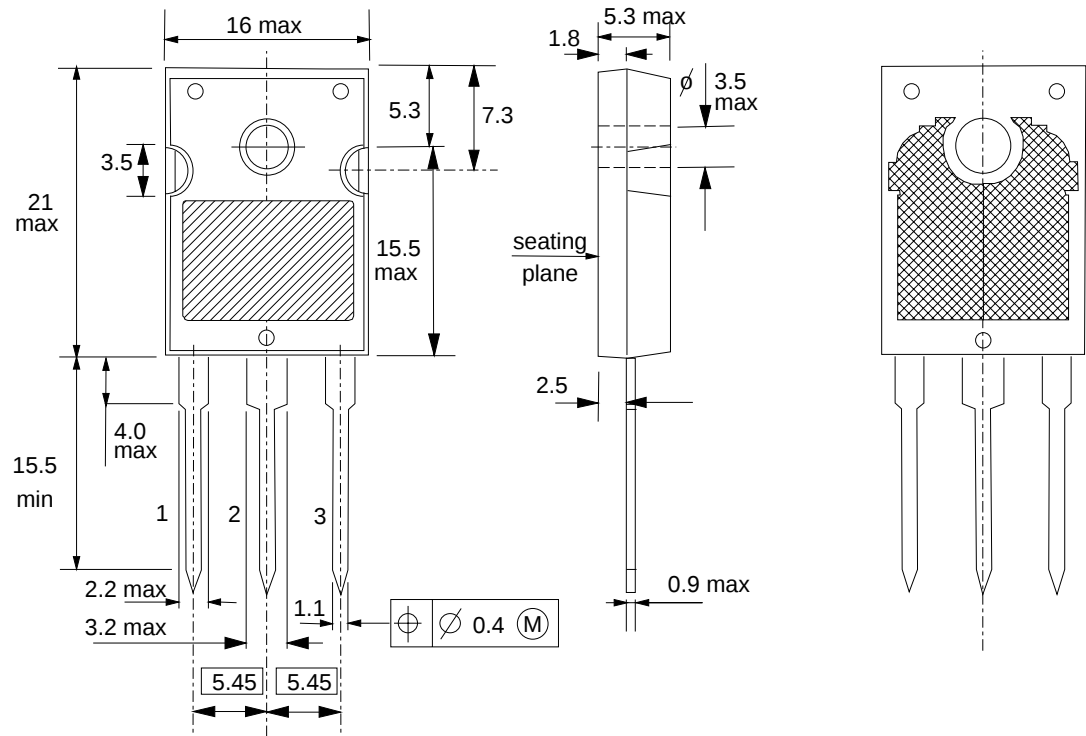
Fig.19. SOT429 (TO247); pin 2 connected to mounting base.
