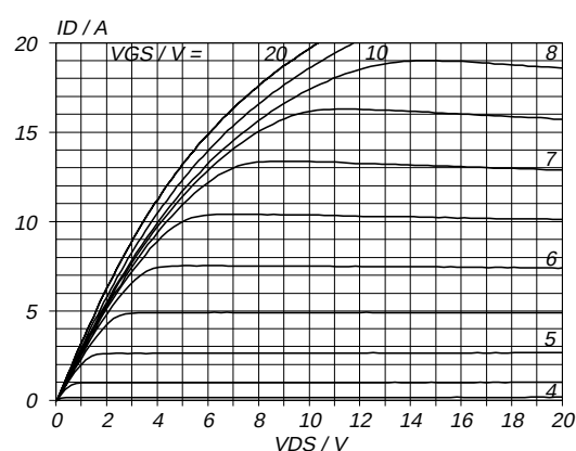
Fig.5. Typical output characteristics. I_D = f(V_{DS}) ; parameter V_{GS}
