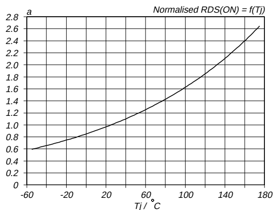
Fig.9. Normalised drain-source on-state resistance. a = R_{DS(ON)} / R_{DS(ON)25\text{ °C}} = f(T_j) ; I_D = 5.9 A; V_{GS} = 10 V
